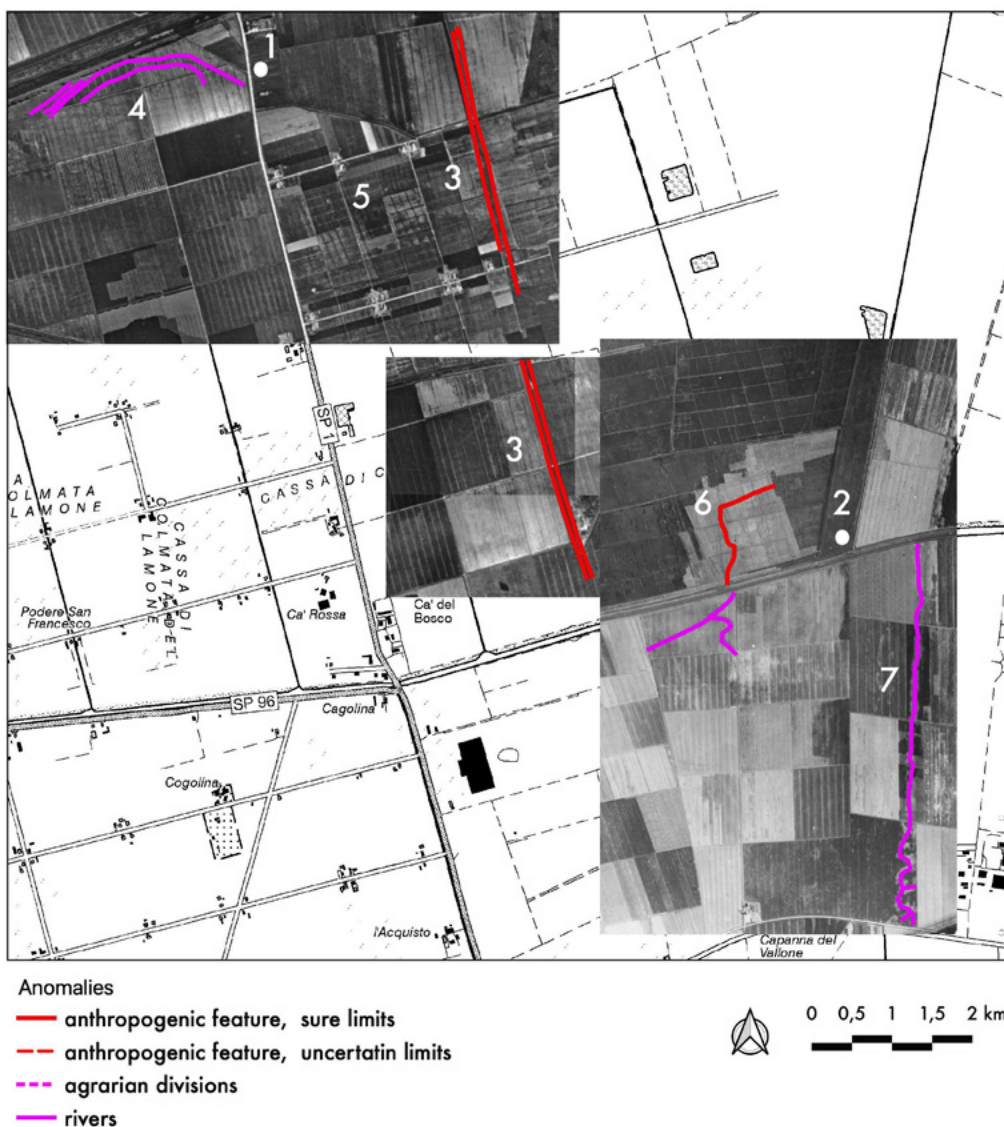
Figure 12. Highlighting of main anomalies near the area of S. Pietro in Armentario (no. 1) and the area of Palazzolo (no. 2): the Padoreno channel (no. 3); fluvial meander (no. 4); rice paddies (no. 5); trail path (no. 6); swale (no. 7).
