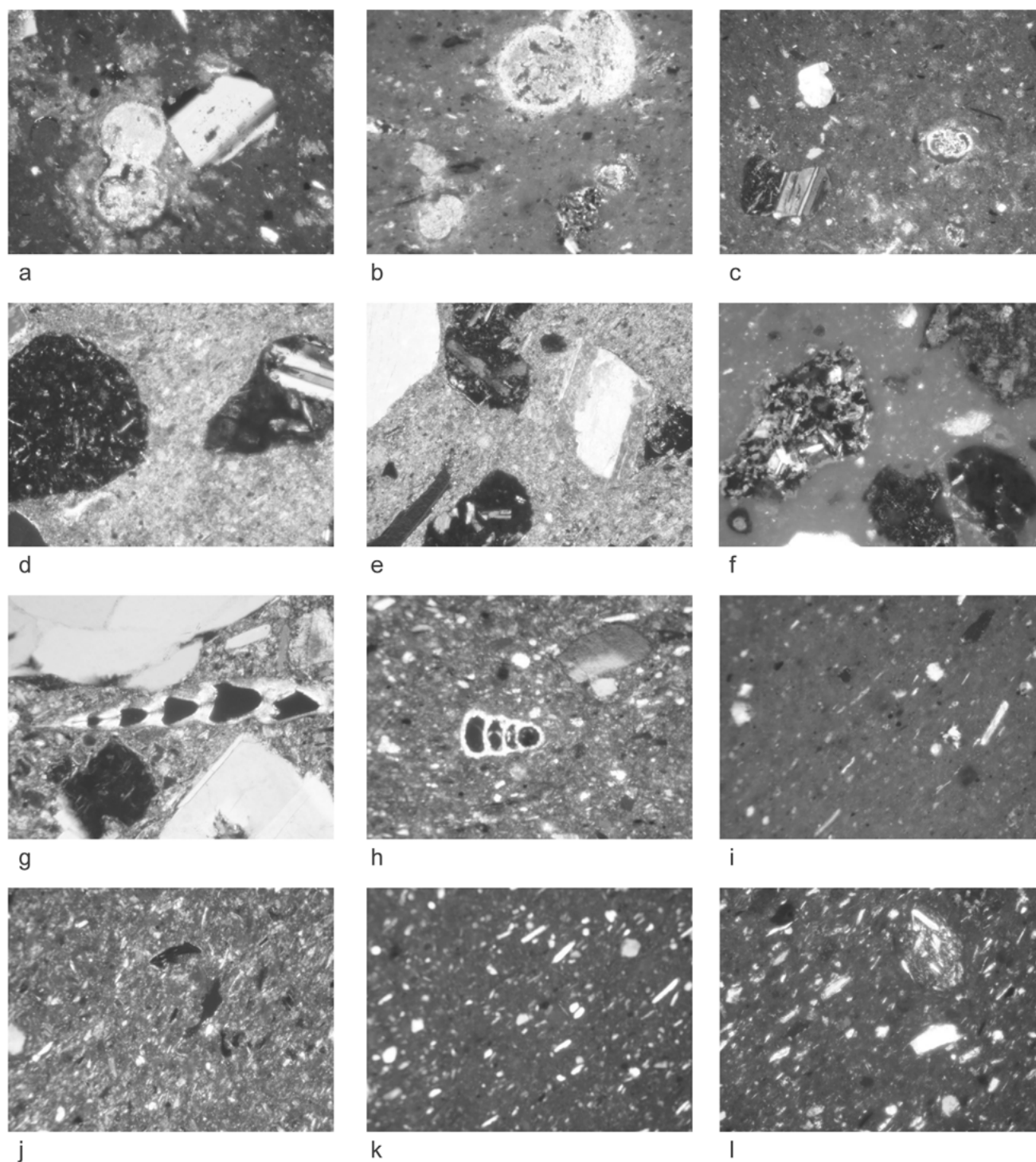
Fig. 1. Photomicrographs of typical micro-fabrics and inclusions (XPL, width of field 0.7 mm): a) lamp of type Esquilino (V729/group 1a) showing microfossil and plagioclase; b) mould (V732/group 1a) with two microfossils and a volcanic rock fragment; c) miniature vessel (V872/group 1a), inclusions as in fig. 1a; d) terra sigillata (V738/group 1a), coarser volcanic inclusions in a lower fired matrix than in figs. 1a–c; e) mould (V733/group 2a), inclusions and matrix as in fig. 1d; f) common ware (V748/group 2b), volcanic inclusions in a high fired isotropic matrix; g) brick (V755/group 3), showing microfossil, plagioclase and pyroxene; h) sigillata Puteolana (5369), high fired red matrix with fine mica, i) regional imitation of Eastern sigillata (V975) with inclusion of a microfossil and pyroxene in calcareous matrix with fine quartz and mica; j) Production A sigillata (V776), black spots are tiny glass fragments, k) sigillata from Arezzo (4898), high fired red matrix with fine mica; l) Gnathia style pottery (MD4210), inclusion of a micaceous rock fragment in red matrix with quartz and fine mica.
