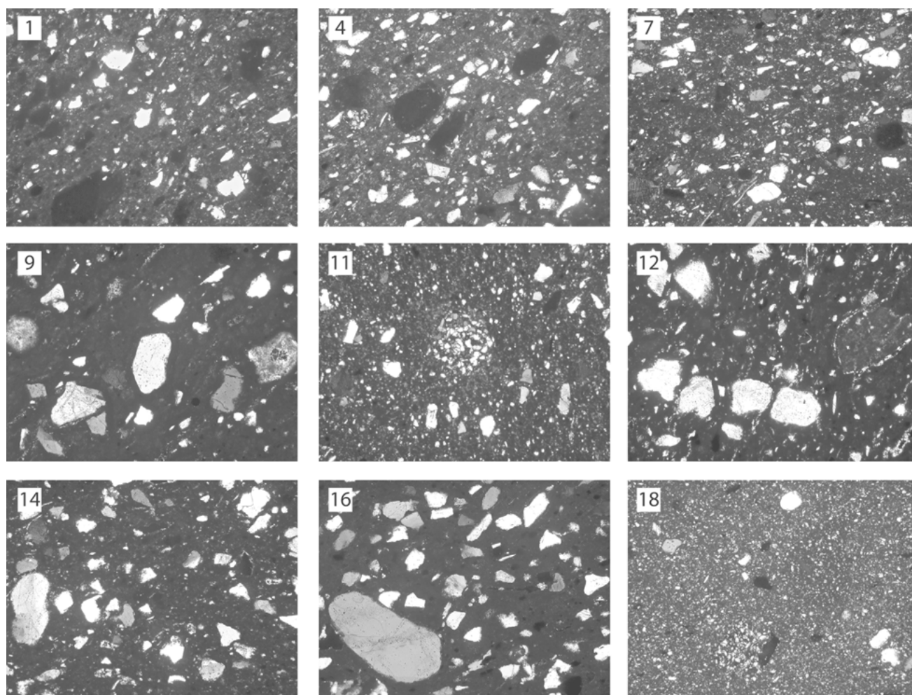
Fig. 4. Microphotographs of the fabrics of selected samples; crossed polars, actual dimensions 1.3×1 mm (C. Capelli).
